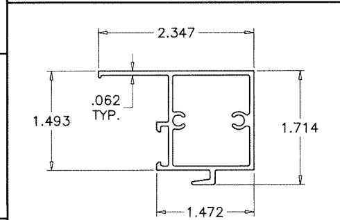
⑦A VENT INTERLOCK W/O HANDLE
