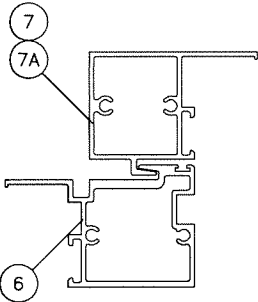
FIX. STILE W/O REINF.
